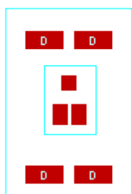
DIRECTFET-MZ
