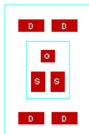
DIRECTFET-MN
