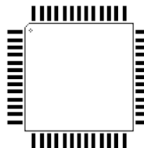
CQFP52
