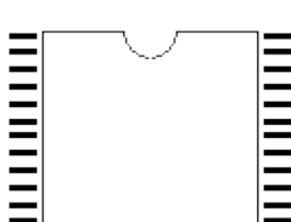
MO-021/24
