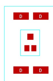
DIRECTFET-MQ
