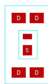
DIRECTFET-SQ
