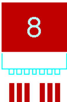
DPAK-7
