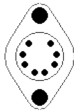
T03-8
