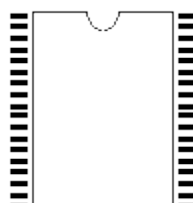
MO-021/36
