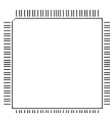
CQFP128
