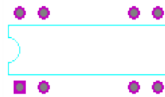
RLY-P&B-JWD
