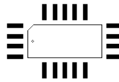
PLCC18/RL
