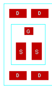
DIRECTFET-MT
