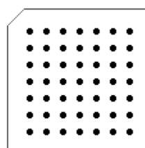
BGA12_49_1.5
