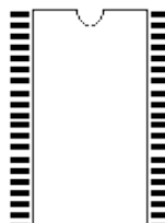
MO-020/40
