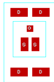
DIRECTFET-MX
