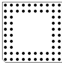
PGA64
