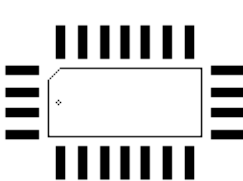
PLCC22/R
