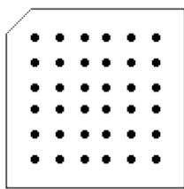
BGA10_36_1.5
