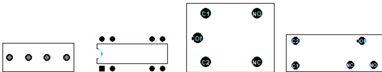
RLY-MAGNECRAFT-A
